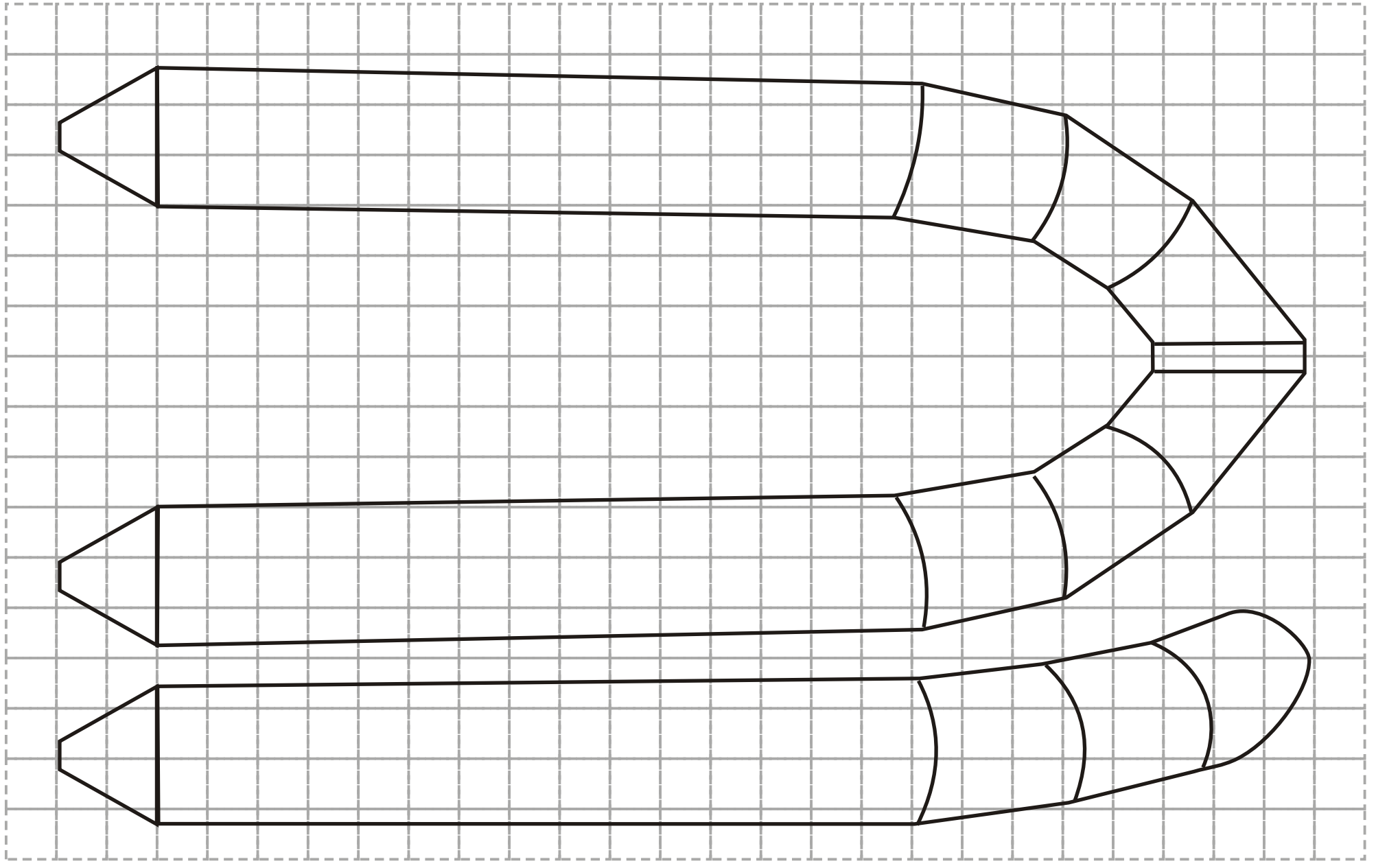
Eurocraft GB Ltd Segmented RIB collar templates
